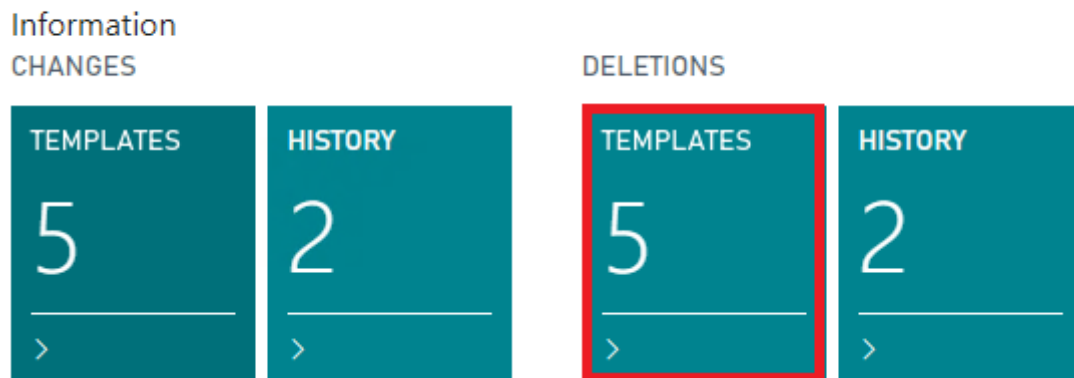
Figure 19: Deletions Templates
