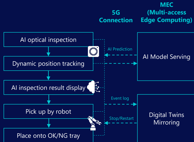
Process Flow
