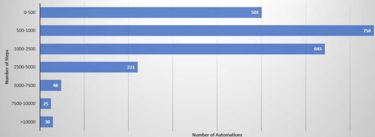
Number of Steps per Automation
