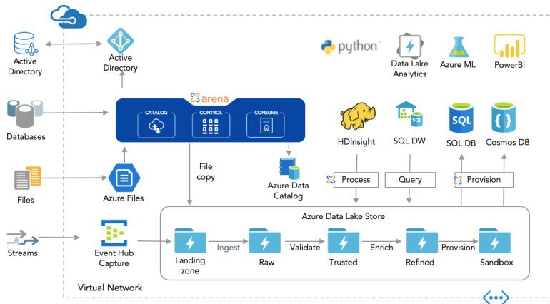
Solution Architecture for Native Azure Data Lake with Arena
