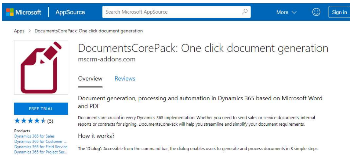
Figure 3: AppSource – DocumentsCorePack
