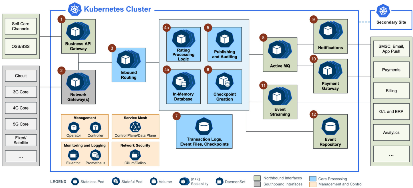
Figure 1: MATRIXX Digital Commerce Platform Cloud Native Architecture
