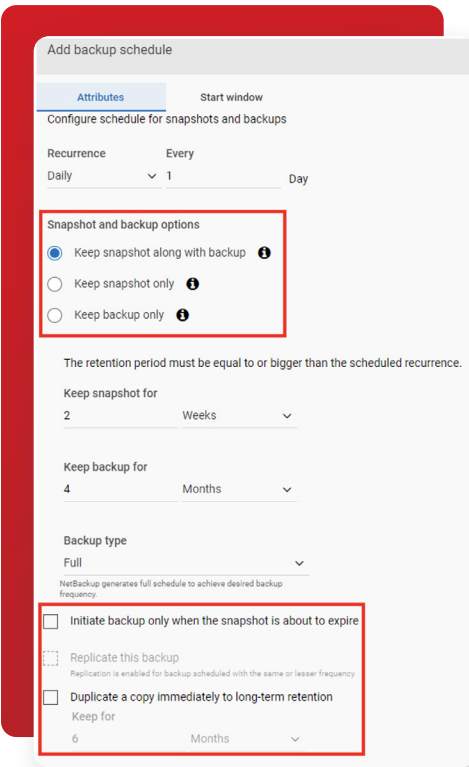
Figure 14: Configuring NetBackup snapshot and backup options.
