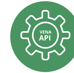
PUBLIC API
