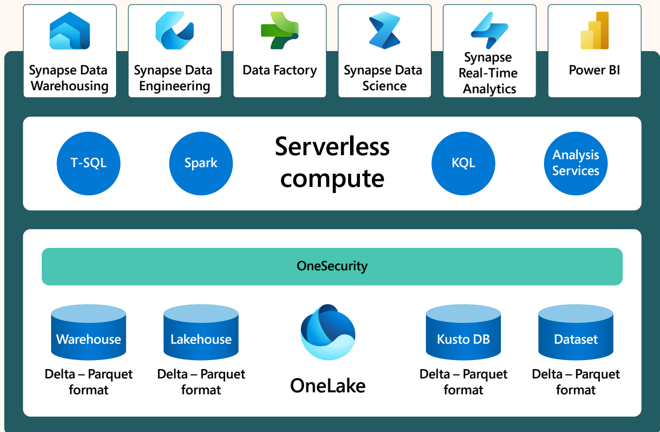
Figure 1: Microsoft Fabric overview
