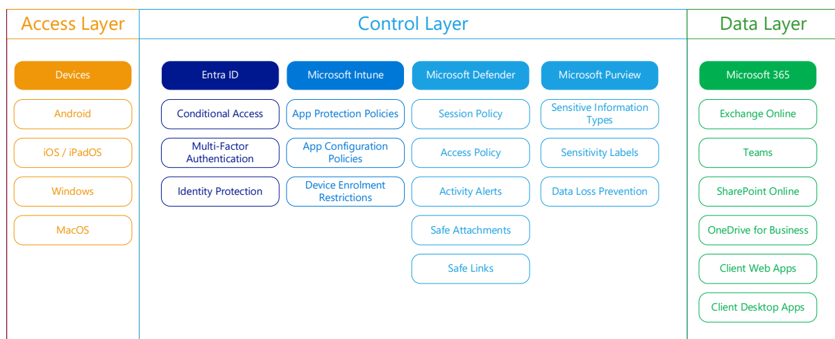
Figure 3: Microsoft 365 Blueprint components
