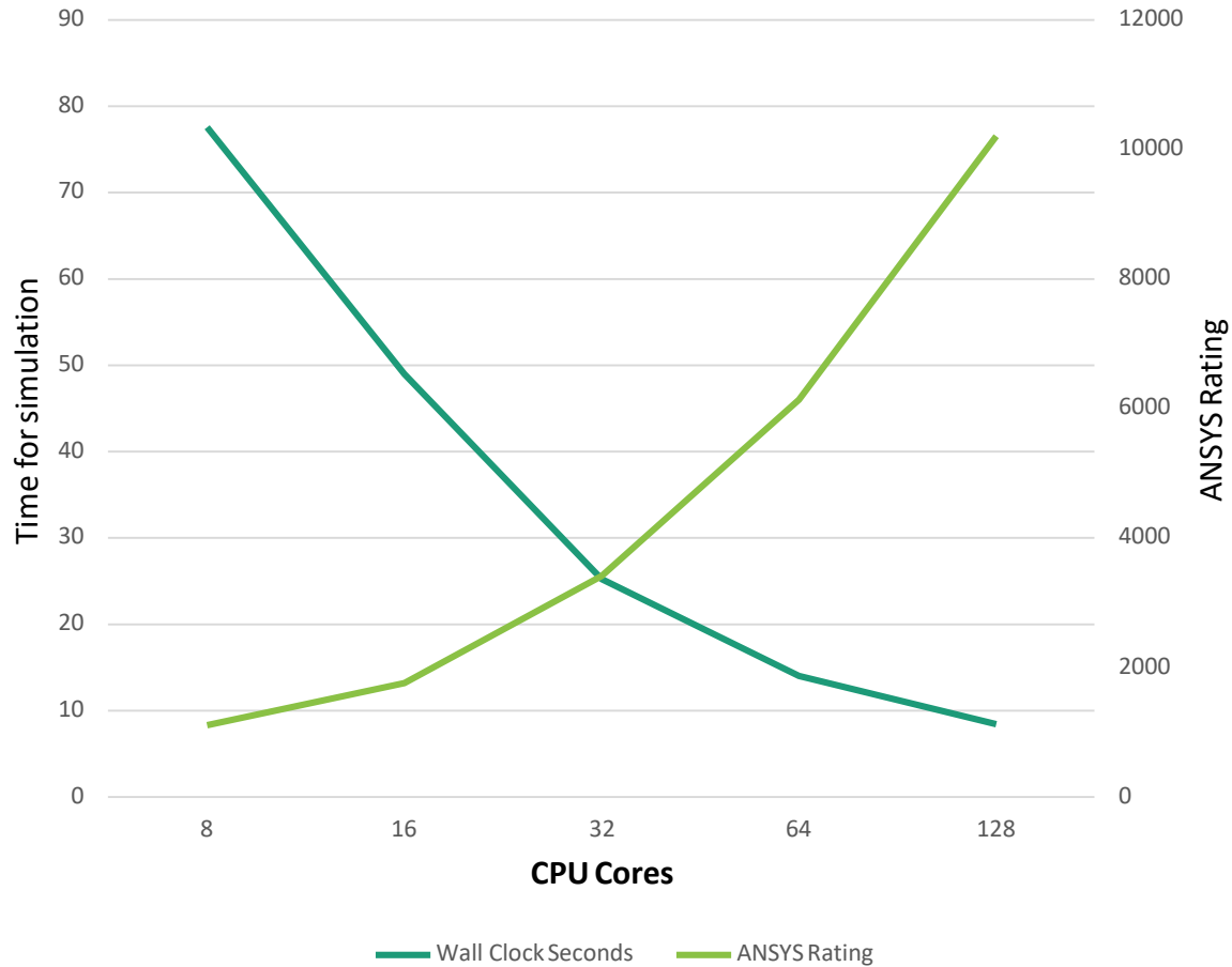
ANSYS Fluent (Sedan_4m): SyncHPC Performance
