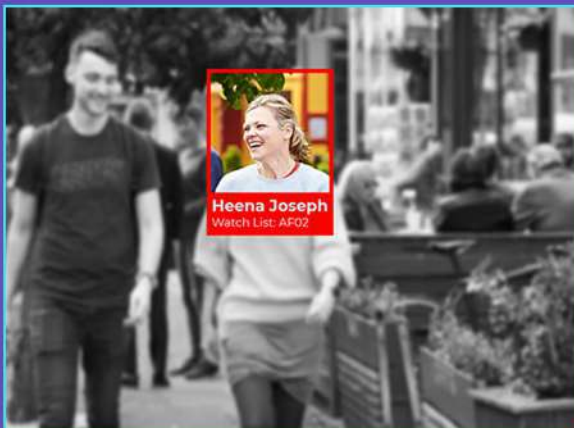
Face Detection
