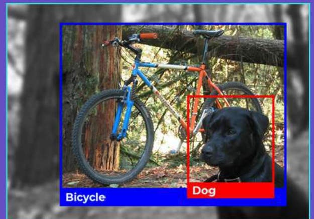
Object Detection
