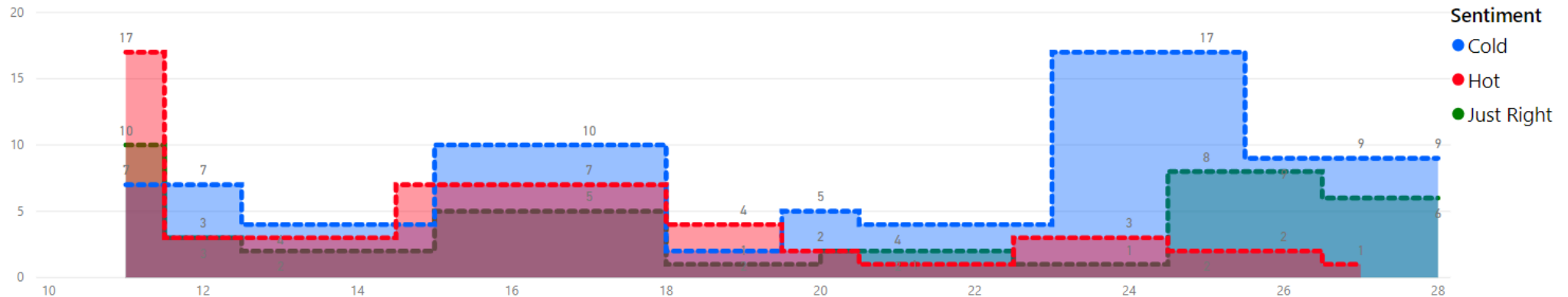
Temperature Sentiment by Time of Day
