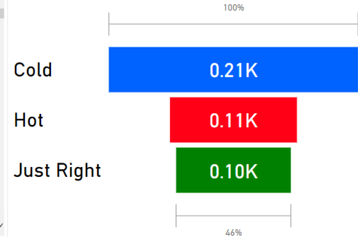
Voltage Usage During Sentiment
