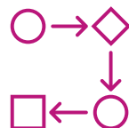
Solution Architecture
