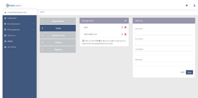
Admin Page
