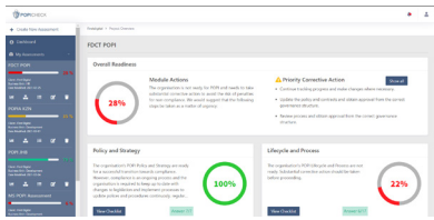
Dashboard
