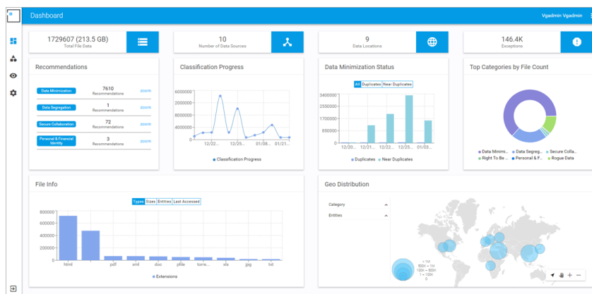
Auto-Classification Dashboard
