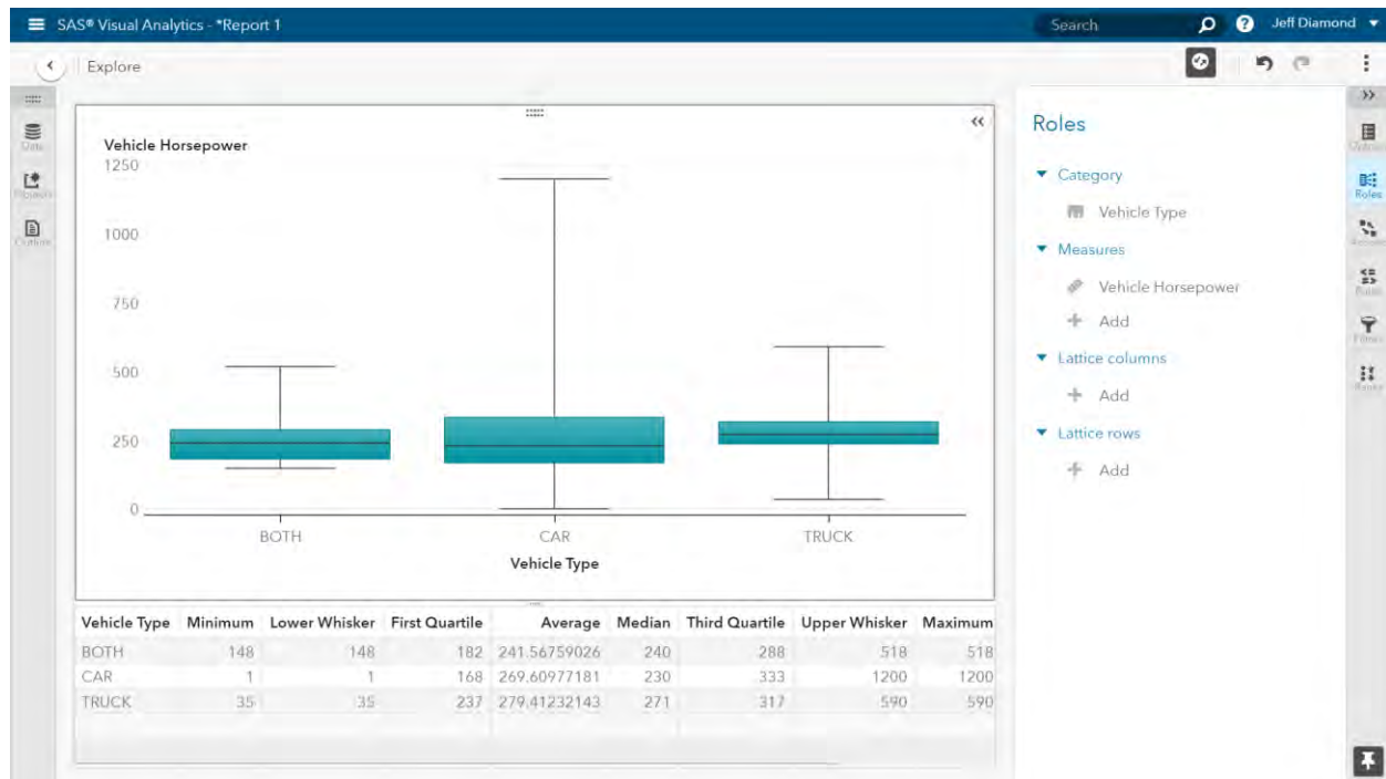
Display 31. Explore Mode, Supplemental Table
