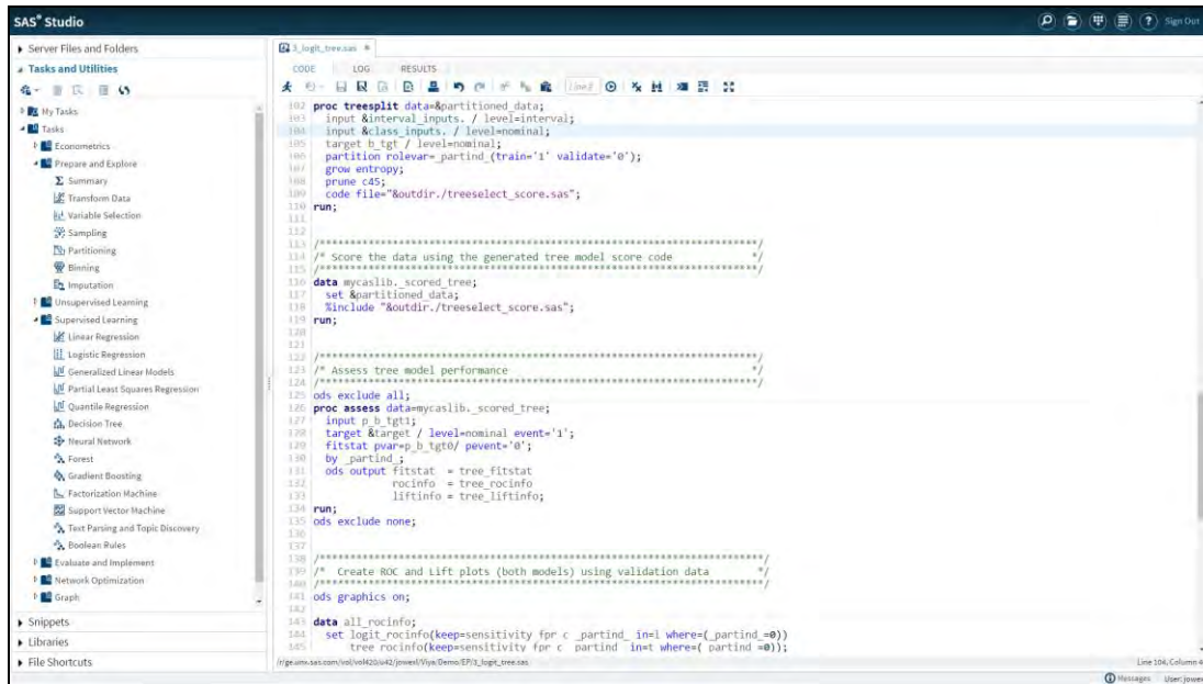
Figure 4. Access the SAS Viya Methods Using the SAS Language within SAS Studio
