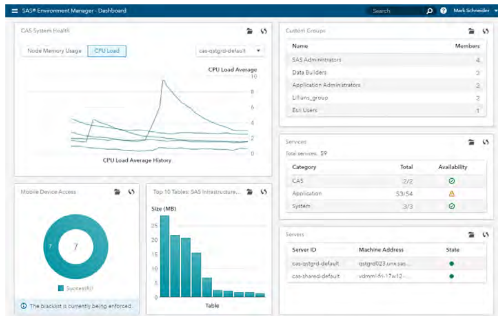
Figure 4. SAS Environment Manager Dashboard
