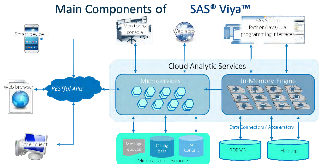
Figure 2. SAS Viya High-Level Architecture
