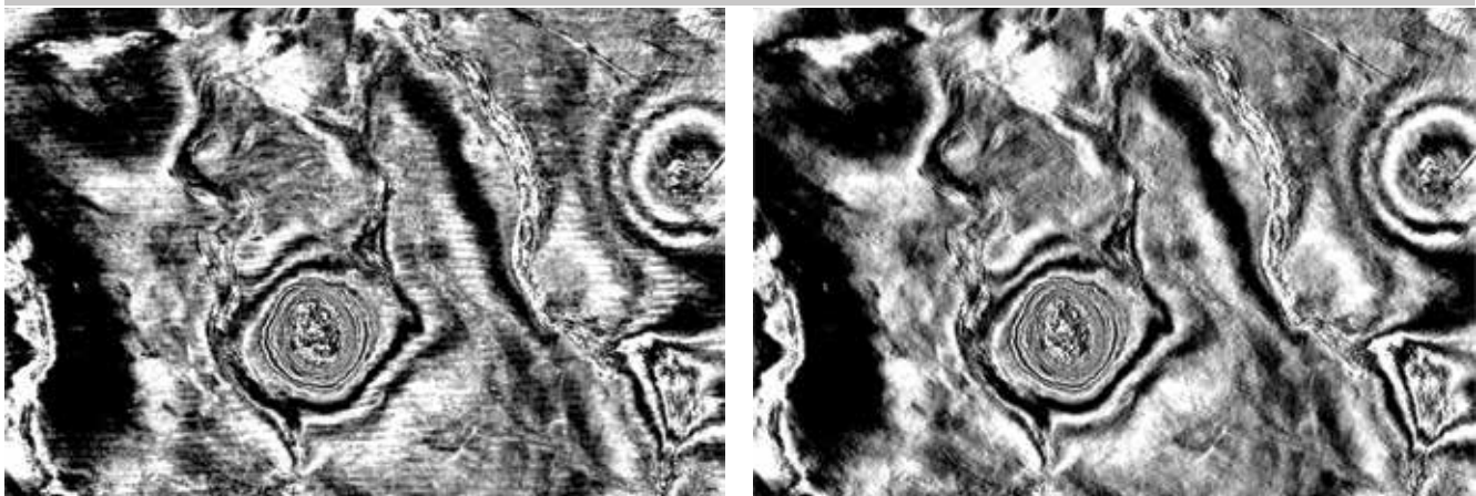
02. Timeslice (400 ms) before (left) and after (right) acquisition footprint removal.
