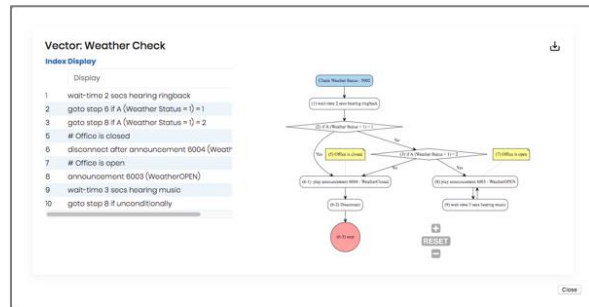
Call Flow Visualization
