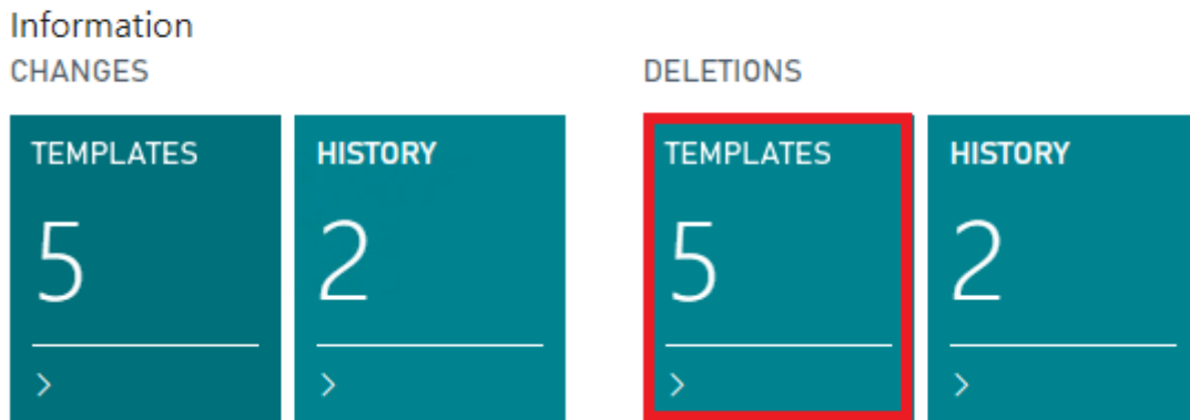
Figure 19: Deletions Templates
