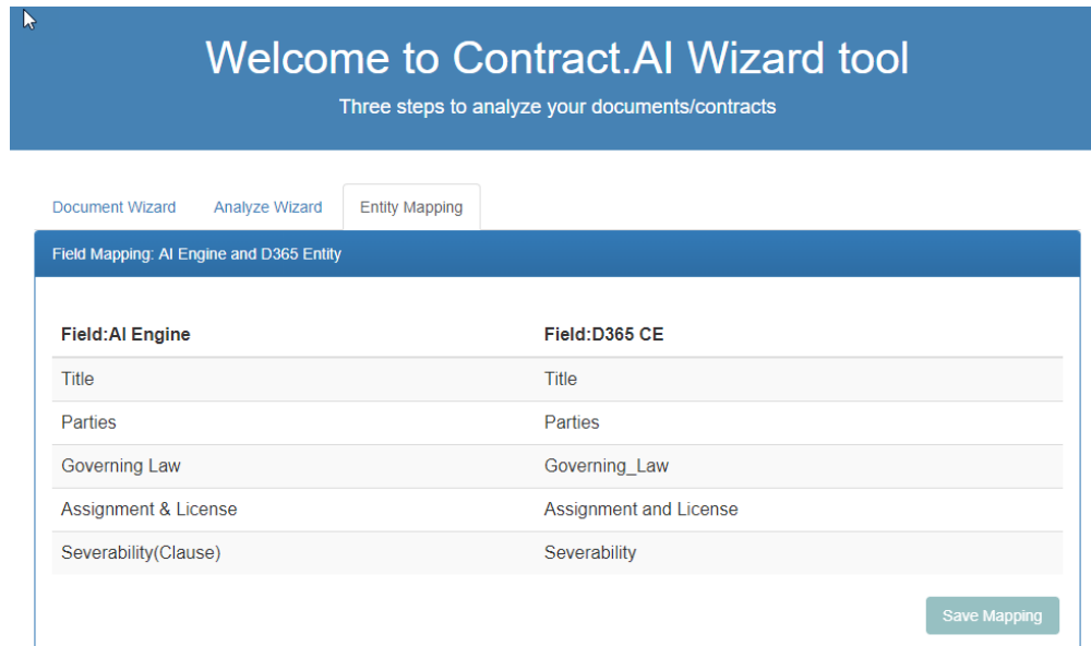
Fig 4: AI engine and D365 CE field mapping
