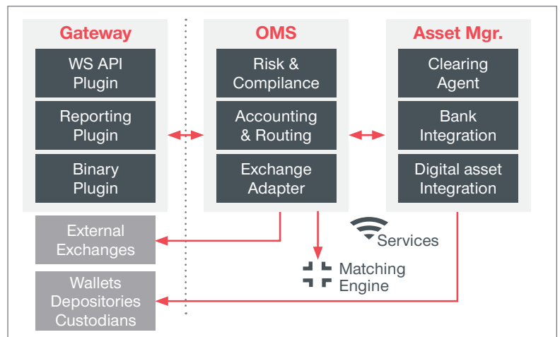
AlphaPoint System System diagram
